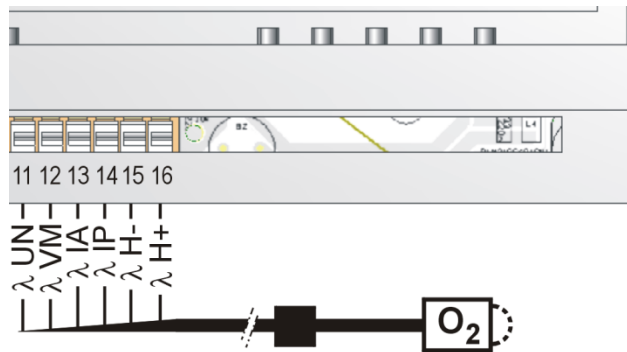
Fig 6.7 Connecting the probe to the module
